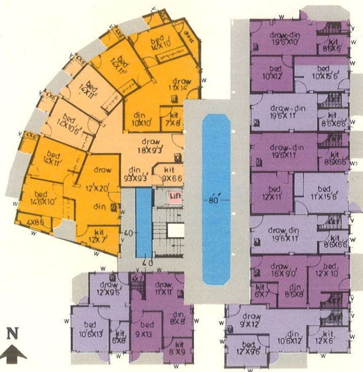
PLAN FOR THIRD FLOOR
