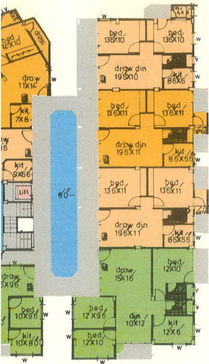
PLAN FOR FIRST AND SECOND FLOOR
